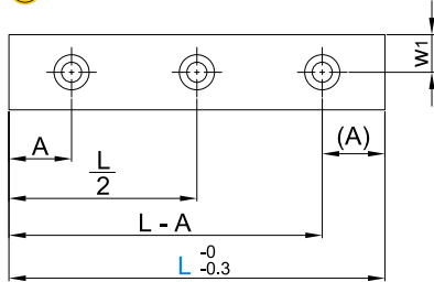
! Mounting Bolt Holes : 3
