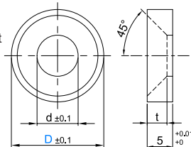
Model: 25STRT Stopper Ring for Tapered Bolt
