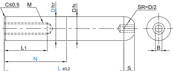
Model: 25AGHXS Tapped + Hex Socket Stepped Type
