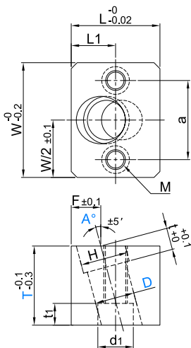
Model: 25AGRWS Double Bolt Type
