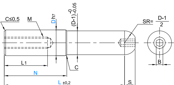
Model: 25AGHXS Tapped + Hex Socket Stepped Type
