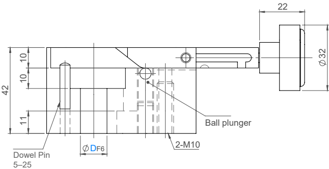
For round punch
