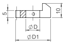
For shaped punch
