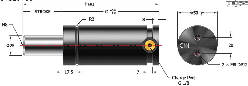
Charging Pressure
