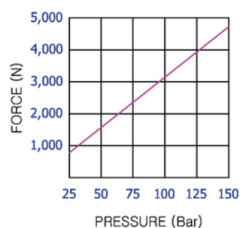
Charging Pressure
