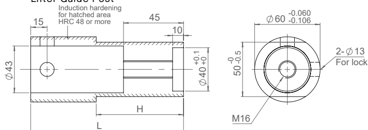
Model: 25LGP-T Lifter Guide Post
