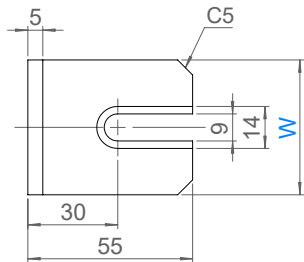
Model: 25SKIL-B Lift Block
