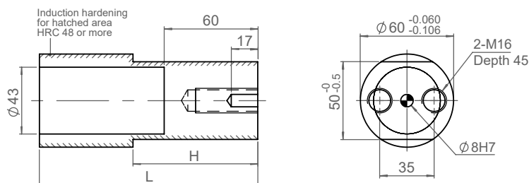
Model: 25LGPP-P Lifter Guide Post
