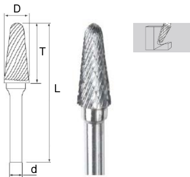
Model: 16SL Round Cone
