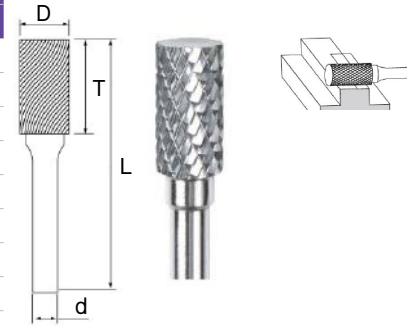
Model: 16SA Cylindrical
