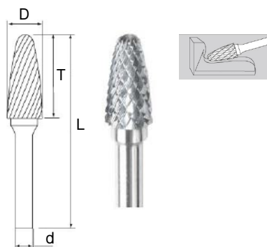
Model: 16SF Round Tree
