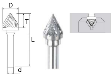
Model: 16SK Cone 90°
