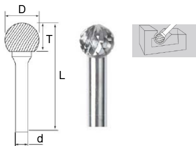
Model: 16SD Ball End
