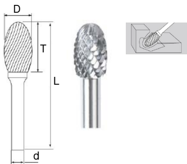
Model: 16SE Oval
